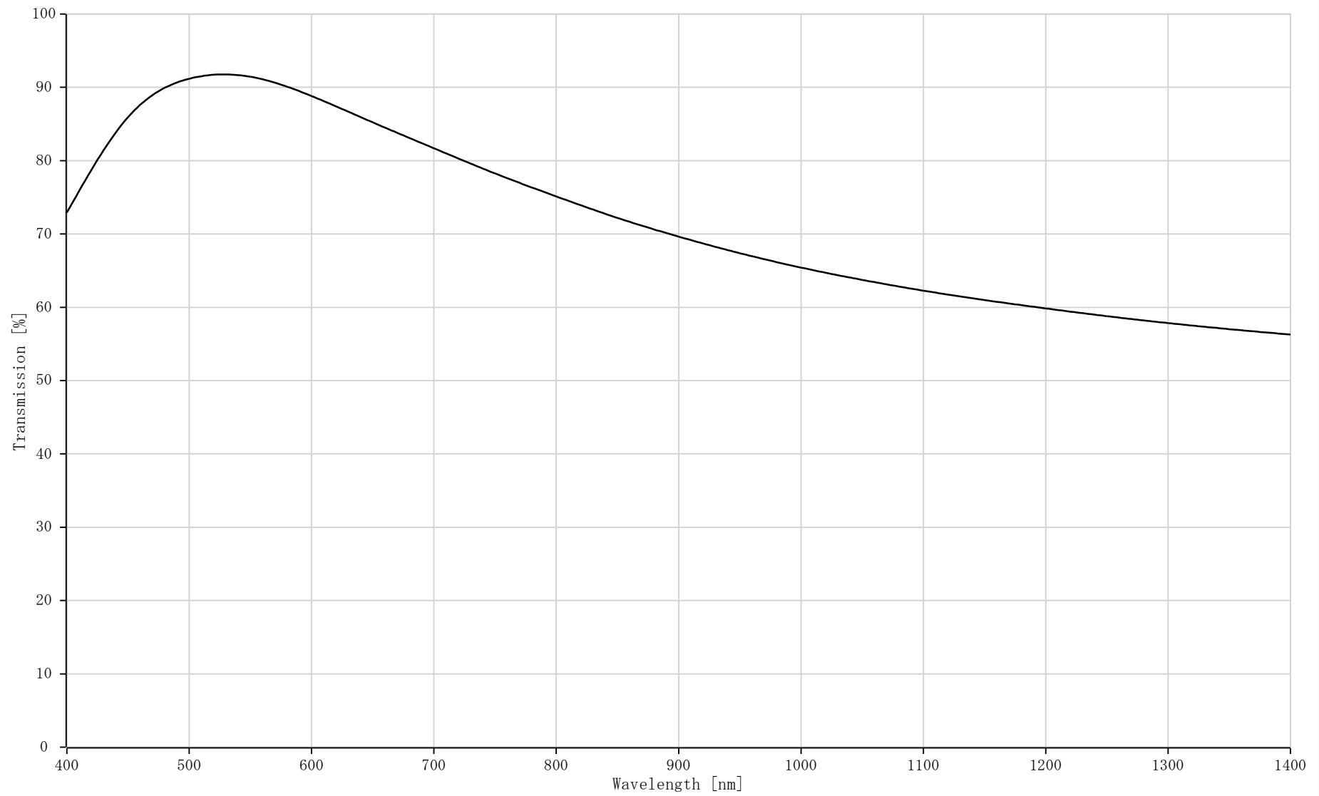
LM50EC-IR Transmission
